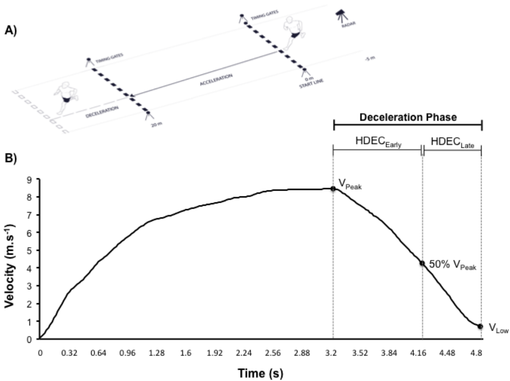
Figure 1. (a) Maximal horizontal deceleration test and (b) example of instantaneous velocity-time profile showing deceleration phase following manual processing with Stalker ATSTM system software. Note: V_{max} = maximum velocity defining start of deceleration phase; 50\% V_{max} = 50% of maximal velocity separating early and late deceleration phases; V_{low} = lowest velocity defining end of deceleration phase; HDEC_{Early} = early deceleration phase representing time between V_{max} and 50\% V_{max} ; HDEC_{Late} = late deceleration phase representing time between 50\% V_{max} and V_{low}
